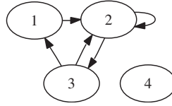
FIGURE 1. A finite directed graph G
