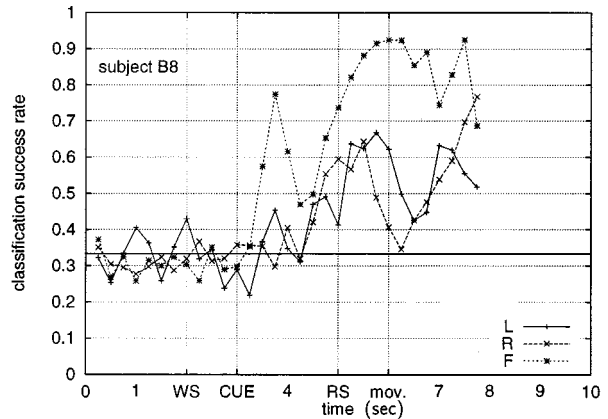
Fig. 4. Classification success rates for individual events: left finger (L), right finger (R), and right foot (F), for subjects A4, B6, and B8. Rates shown are the number of correctly recognized trials of event X divided by the number of trials of event X in the test set.
