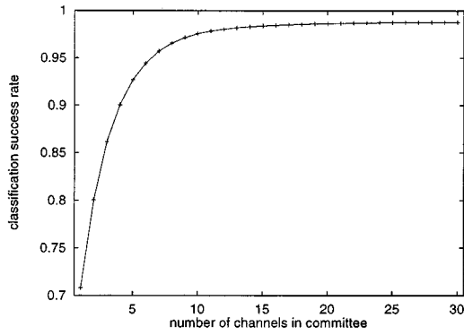
Fig. 2. Classification success averaged over trials from the validation set as function of committee size. The results shown were obtained by averaging over 5000 random partitions of available trials in training, validation, and test set. Laplace filtered data (Section III-D1) from subject A4 were used, analyzed as AR(10) coefficients computed in the period from 5 to 6 s. No bandpass filter (Section III-D2) was applied.
