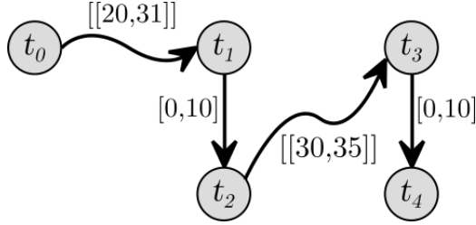
Figure 1: An STNU representation of Dr. V's experiment.
