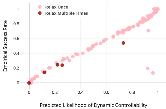
Figure 8: Dispatch Success Rate vs. Approximate LDC
