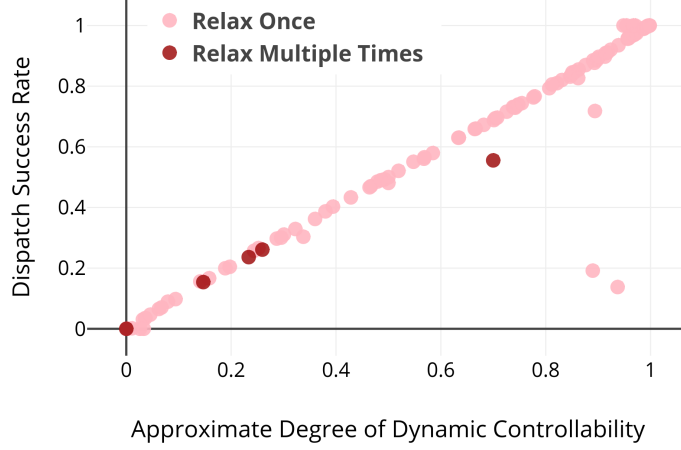
Figure 6: Dispatch Success Rate vs. Approximate DDC
