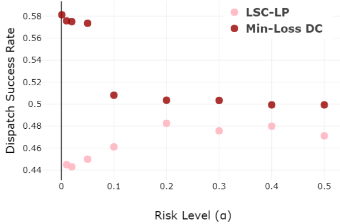
Figure 9: LSC-LP and MIN-LOSS DC Success Rates Across Risk Levels on CAR-SHARING
