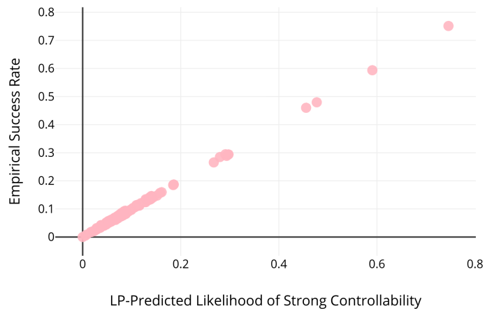
Figure 7: LSC success PSTN
