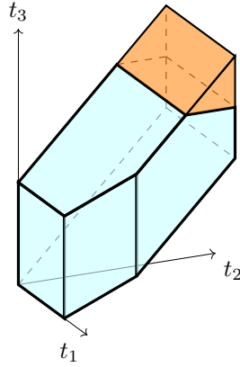
Figure 2: The polytopes associated with network \mathcal{S} .
