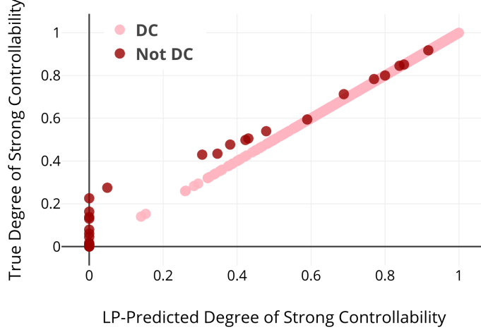
Figure 5: True DSC vs. DSC-LP.
