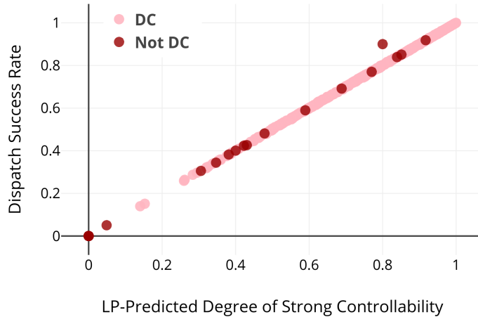
Figure 4: LP-Strong Decision vs. Predicted DSC
