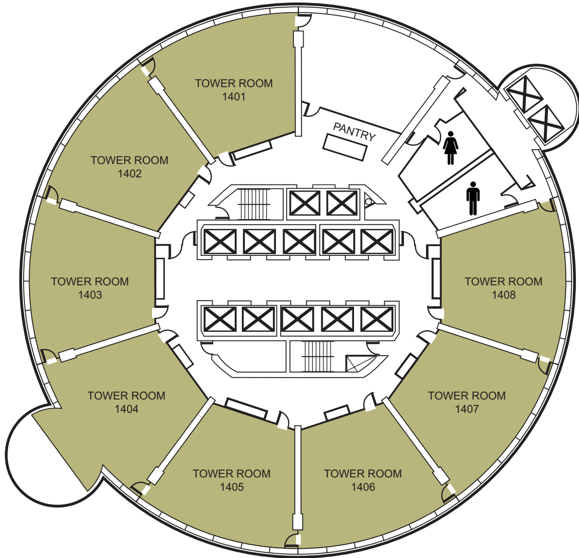
FOURTEENTH FLOOR
