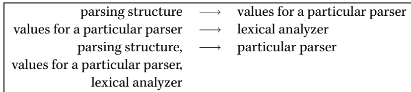
Figure 1: Module Dependencies
