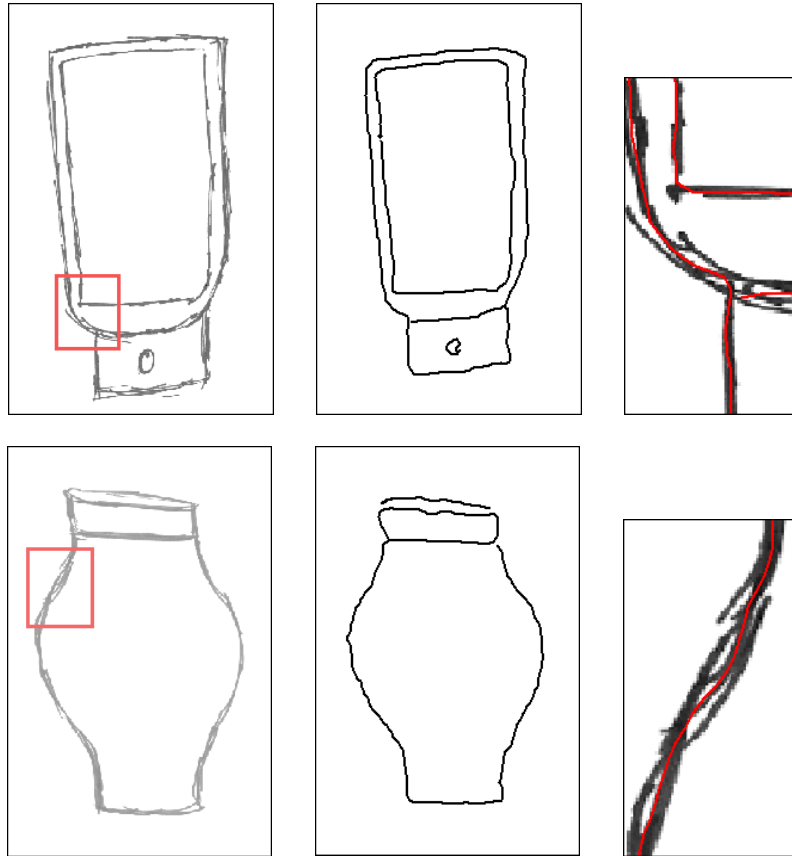
Figure 10: The vector results obtained after applying the proposed scribble simplification techniques to two sample scribbles. In each example, the rightmost figure shows the Kalman Filter result super-imposed on the original scribble for the section highlighted on the original scribbles.
