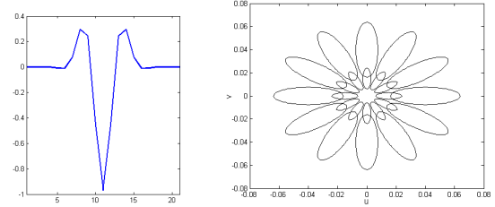
Figure 5: The Gabor filter that detects inter-line gaps. (a) The filter profile (b) the spatial-frequency domain coverage of the filter bank. (Note the scale difference with respect to Figure 3)
