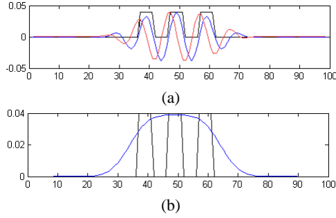
Figure 2: Response of a Gabor filter with wavelength \lambda = 10 for a sequence of three bars. A phase of \phi = 0 radians (blue plot in (a)) responds to the bar centres, a phase of \phi = \frac{\pi}{2} radians (red plot in (a)) gives better response at the bar edges while the the Gabor energy (b) combines the two responses giving a continuous response over all over-traced regions.
