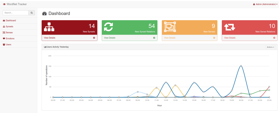
Figure 2: Tracker dashboard.
