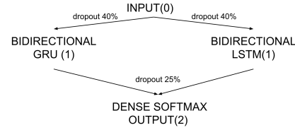
Figure 1: Branched bi gru-lstm architecture.
