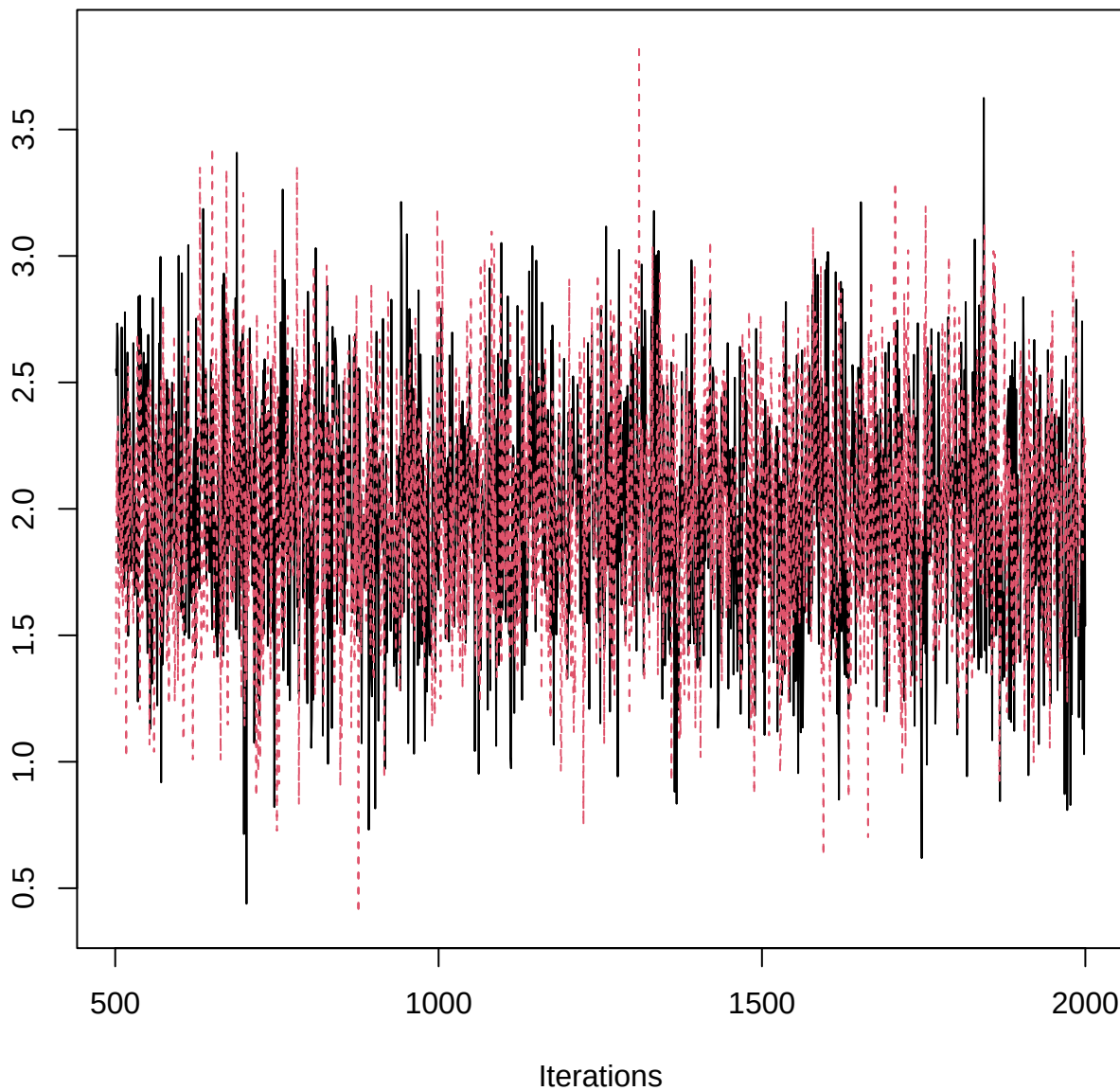
Trace of \mu
